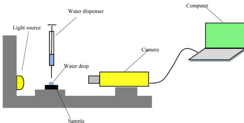
Fig. 4. Scheme system to measurement of contact angle
