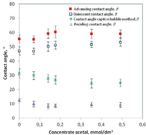
Fig. 6. Summary of the contact angle values of copper-bearing shales obtained using the sessile drop and captive bubble methods in function of acetal solution concentration
