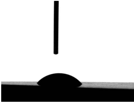
Fig. 1. Example of quiescent contact angle measurement
