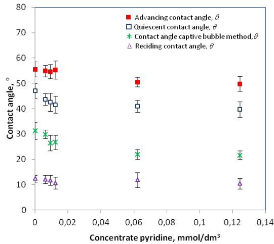
Fig. 5. Summary of the contact angle values of copper-bearing shales obtained using the sessile drop and captive bubble methods in function of pyridine solution concentration
