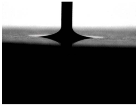
Fig. 3. Example of receding contact angle measurement
