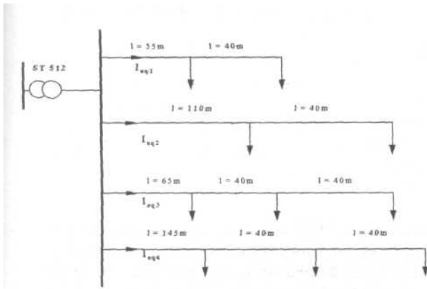
Fig. 3. The exemplary segment of urban distribution low voltage network
