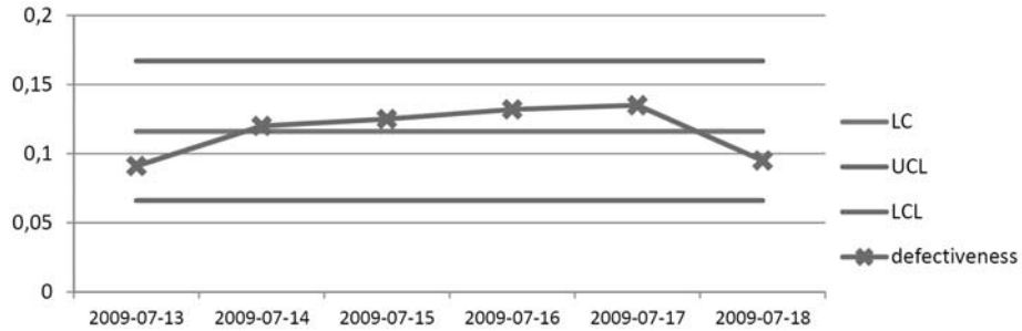
Fig. 9. Control cards p – production errors – hearing aids BTE – week 29 year 2009
