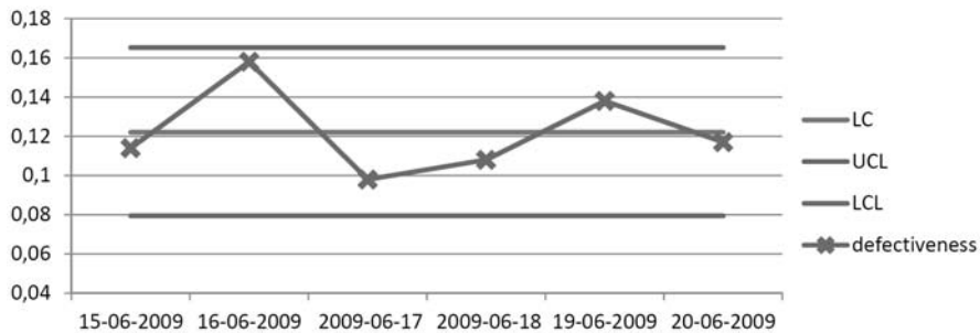
Fig. 5. Control cards p – production errors – hearing aids BTE – week 25 year 2009
