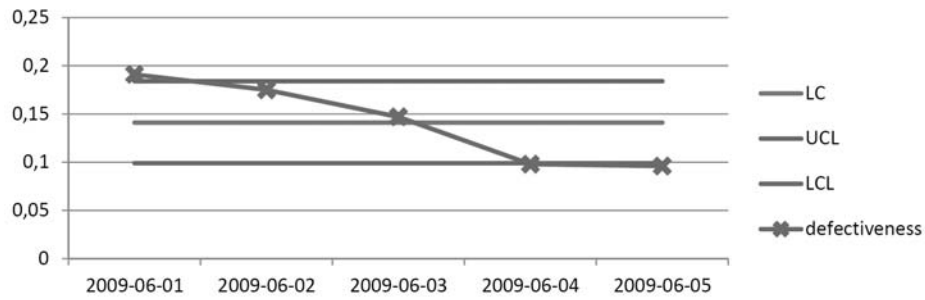
Fig. 3. Control cards p – production errors – hearing aids BTE – week 23 year 2009
