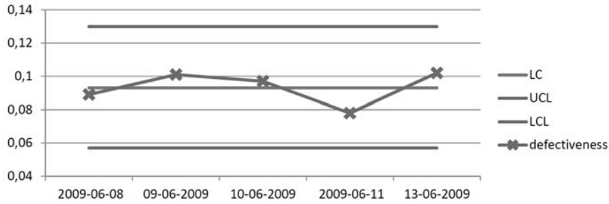
Fig. 4. Control cards p – production errors – hearing aids BTE – week 24 year 2009
