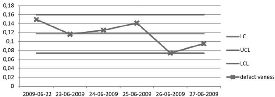
Fig. 6. Control cards p – production errors – hearing aids BTE – week 26 year 2009
