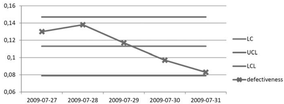
Fig. 11. Control cards p – production errors – hearing aids BTE – week 31 year 2009
