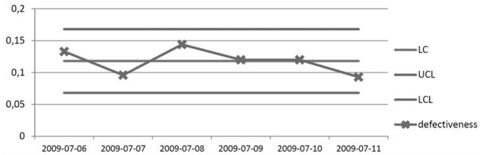
Fig. 8. Control cards p – production errors – hearing aids BTE – week 28 year 2009
