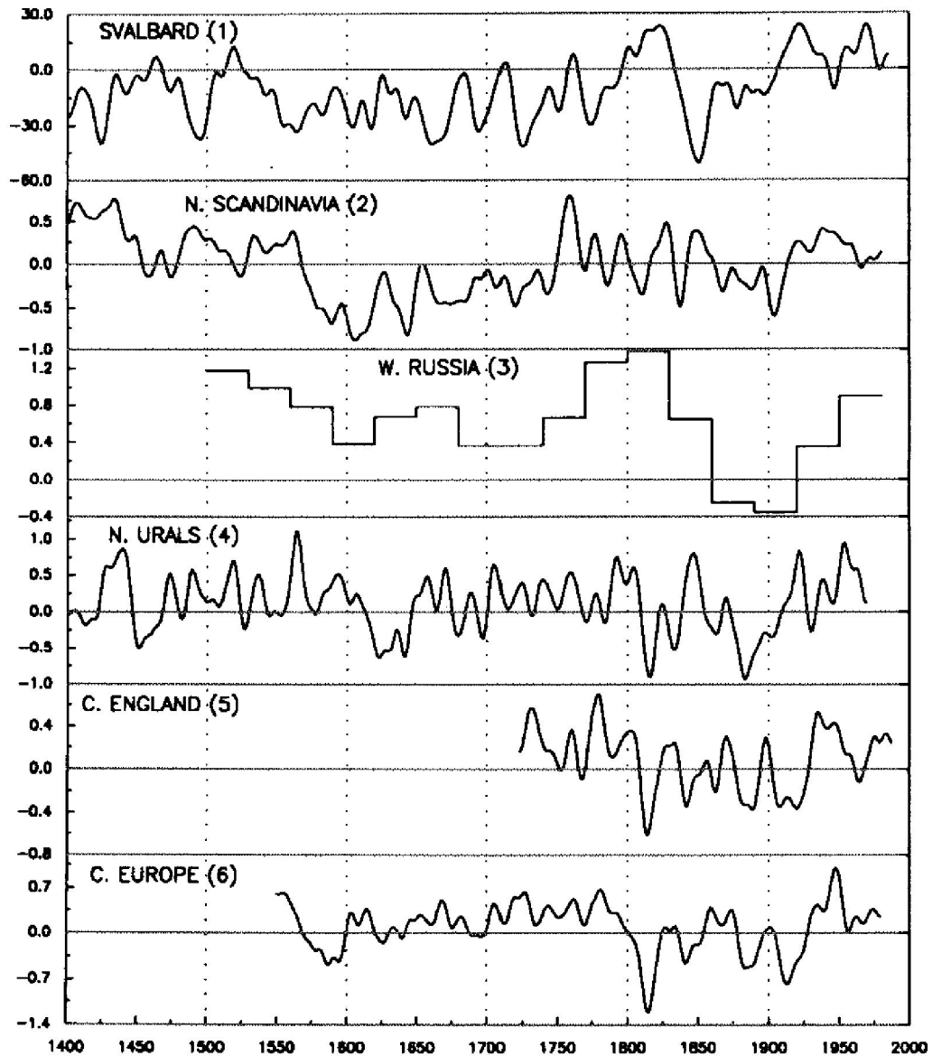
Figure 2 Reconstructed summer temperature anomaly series for Europe (referenced to the mean of each series for 1860–1959). The Svalbard record is of summer melt from the Lomonosov ice cap in Svalbard (Spitsbergen – Tarussov, 1992); the northern Scandinavia series is based on a network of tree-ring density records from Pinus sylvestris at the northern tree-line of Sweden (Briffa, Bartholin et al. , 1990; Briffa, Jones et al. , 1992); the western Russian record is derived from historical documentary sources (Borisenkov, 1992); the northern Urals record is based on tree-ring widths in a set of Larix sibirica trees from the Urals of western Russia (Graybill and Shiyatov, 1992); the central England series is based on instrumental records (Manley, 1959, 1974); the central European record is derived mainly from documentary sources in Switzerland (Pfister, 1985). All units are °C, except for the Svalbard record, which is the core area affected by melting, expressed as percentage departures from the mean.
