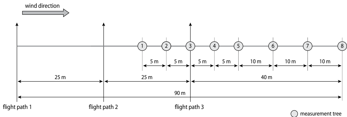
Figure 2. Measurement line pattern in trials on spray drift
