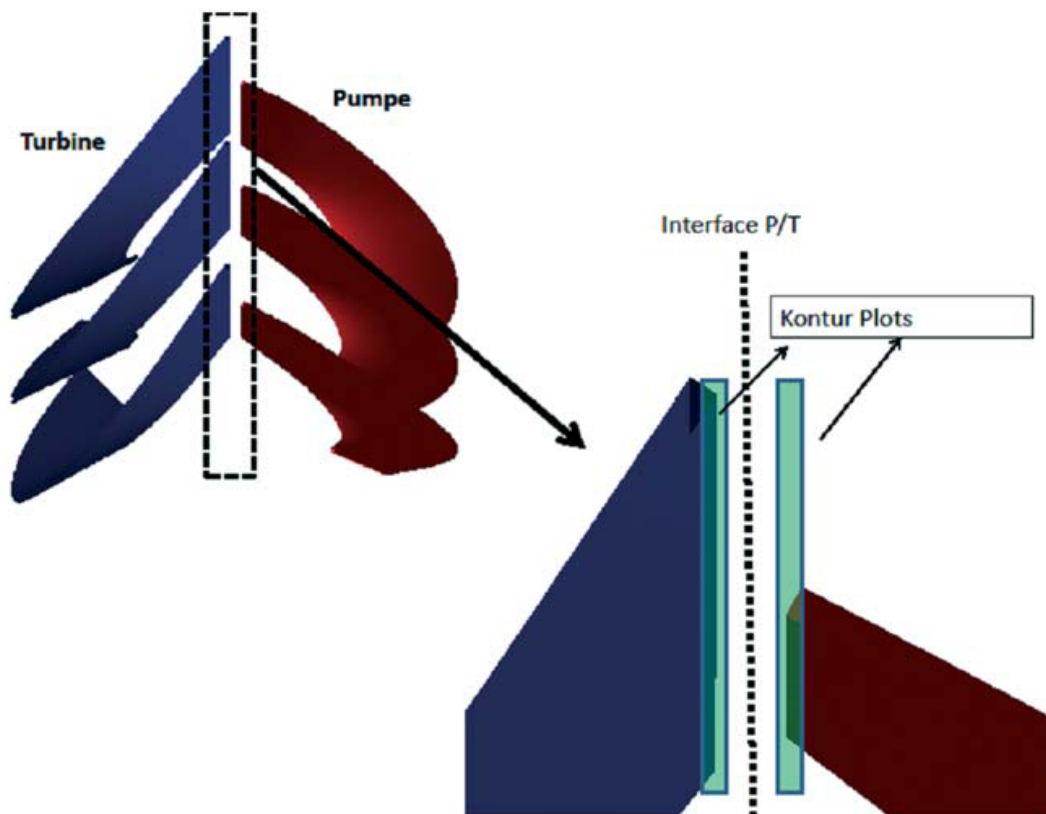
Figure 1. Position of the planes at the pump exit and turbine inlet to describe the blade/row interaction.
