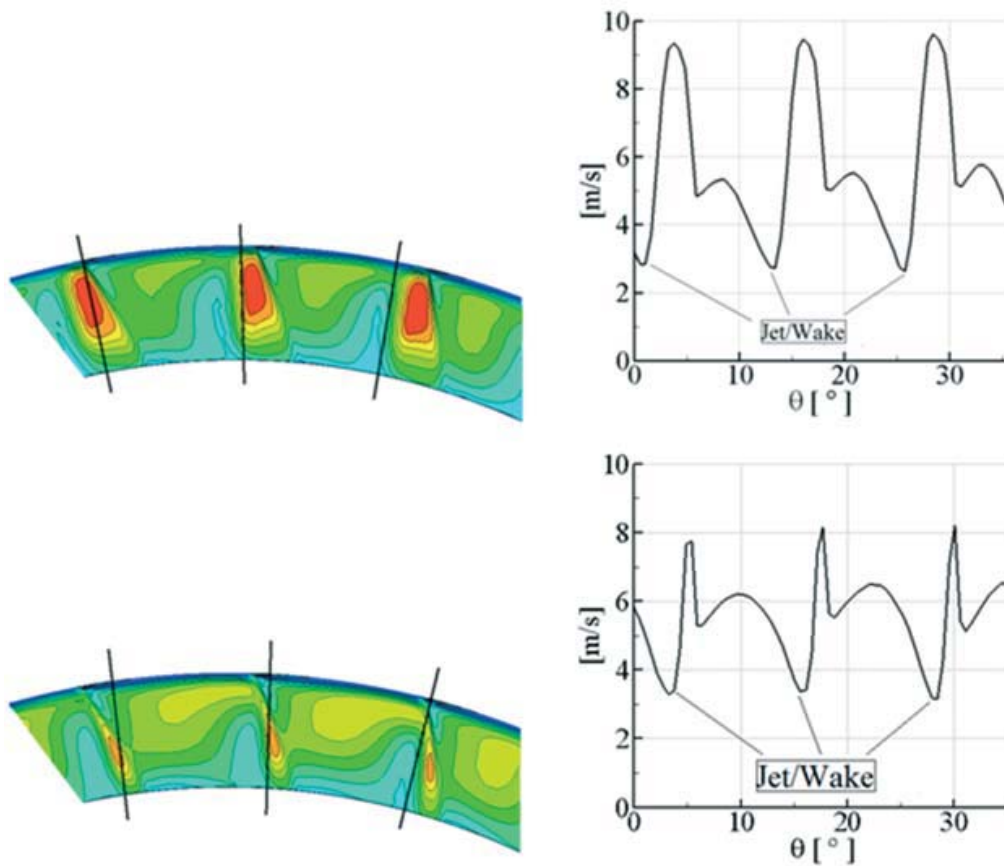
Figure 3. Meridional velocity ( C_m ) contour plot for a period T at the turbine inlet and pump relative position (indicated by the black lines). Rotor relative positions 0 T , 0.2 T , 0.4 T , 0.6 T and 0.8 T .
