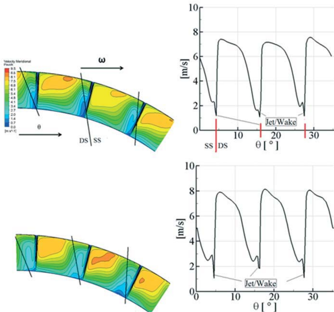
Figure 2. Meridional velocity ( C_m ) contour plot for a period T at the pump exit and turbine relative position (indicated by the black lines). Rotor relative positions 0T , 0.2T , 0.4T , 0.6T and 0.8T .
