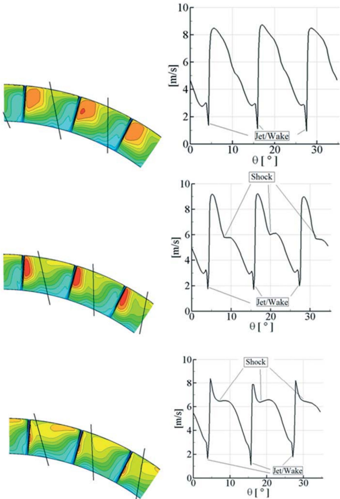
Figure 2. Meridional velocity ( C_m ) contour plot for a period T at the pump exit and turbine relative position (indicated by the black lines). Rotor relative positions 0 T , 0.2 T , 0.4 T , 0.6 T and 0.8 T .
