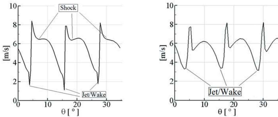
Figure 4. Comparison of the meridional velocity C_m at the pump exit plane (left) and the turbine inlet plane (right) at 0.8 T
