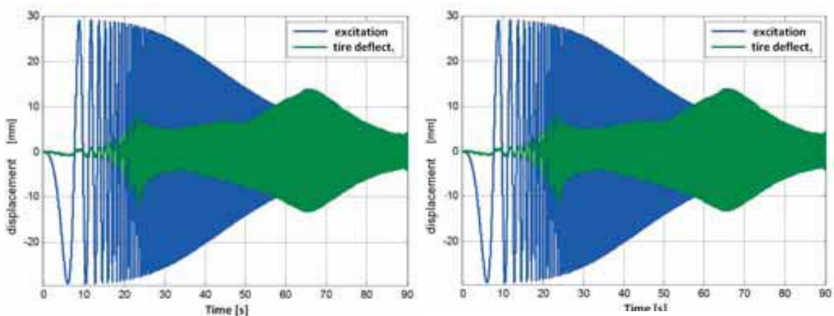
Fig. 7. Examples of direct comparison of measured excitation and response signals in time domain
