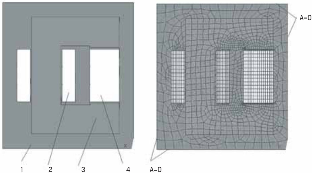
Fig. 6. The model of electric power generator, grid of finite elements and boundary conditions. 1 - air block, 2 - coil, 3 - pole, 4 - permanent magnet
