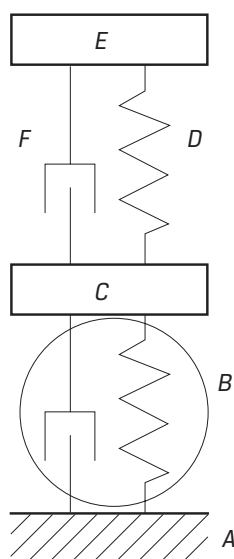
Fig. 4. The modeled set of moving masses for vehicle: the chassis and body and the wheel;
