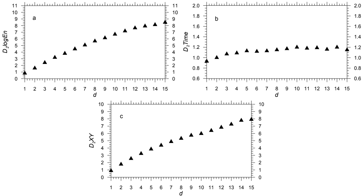
Fig. 3 Correlation dimensions D_2 of the attractors in dependence of Euclidean dimension d of the embedded space reconstructed from the distribution of logarithm of energy (a), time (b), epicycle (c). Tremors generated by mining in Katowice Coal Mine in Poland, in 1985-86.
