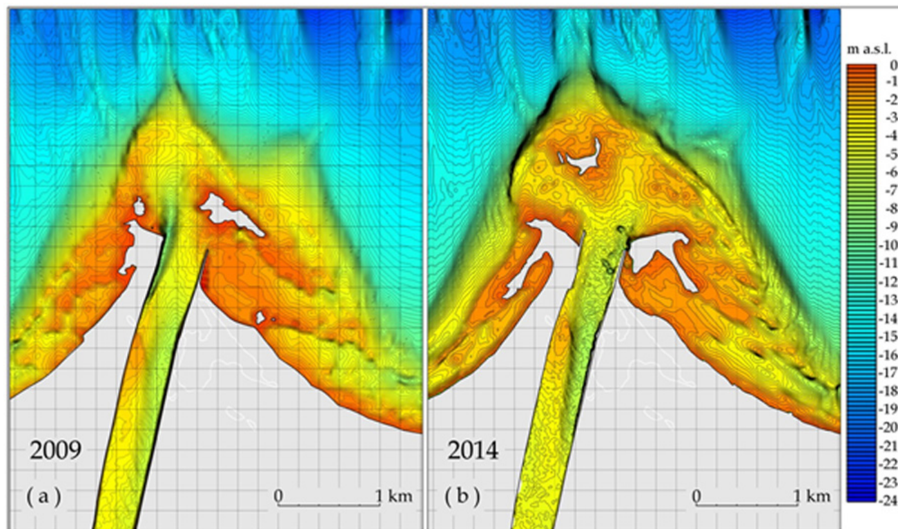
Fig. 2. Bathymetric maps of the Vistula River mouth area based on data obtained in measurement campaigns performed in August 2009 (a) and October 2014 (b). Colorbar scale in meters.
