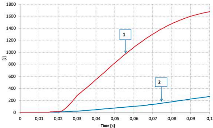
Fig. 6.2. Components of the dissipated motorcycle energy vs. time (1 - E_o , 2 - W_{UM} )
