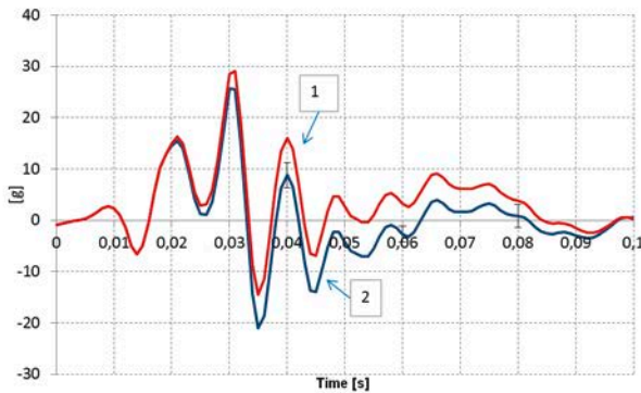
Fig. 5.4. Time histories of a_{MZ} and a_{CZ} (1 - a_{MZ} , 2 - a_{CZ} )
