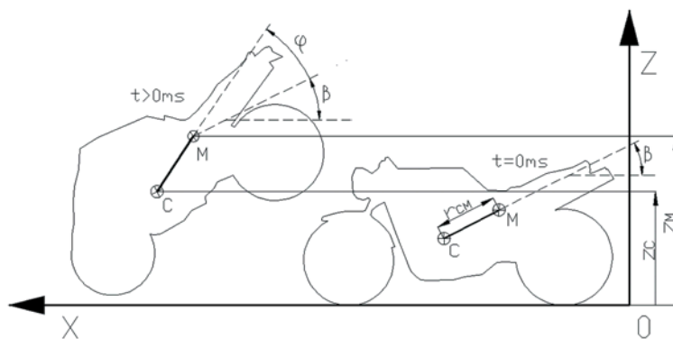
Fig. 5.3. Schematic diagram adopted for calculations of the acceleration of the centre of motorcycle mass
