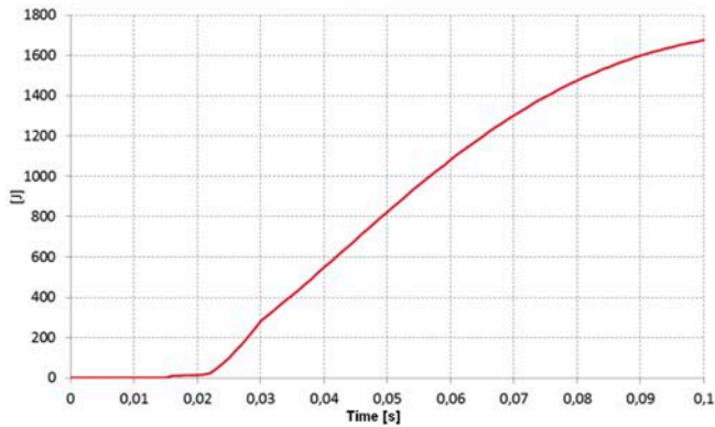
Fig. 6.1. Energy dissipated during the motorcycle rotation vs. time
