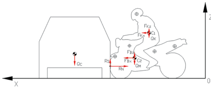
Fig. 4.1. The force system that causes rotation of the motorcycle
