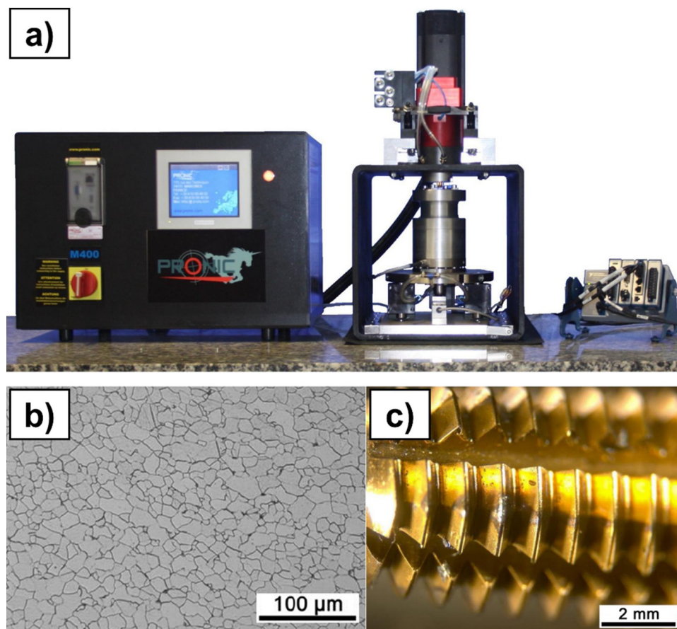
Fig. 2. Overview of the form tapping unit (a). Microstructure of the zinc coated steel used for the form tapping experiments (b). Detail of the TiN coated M12 \times 1.5 6HX tap (c). Figures adapted from [27].
