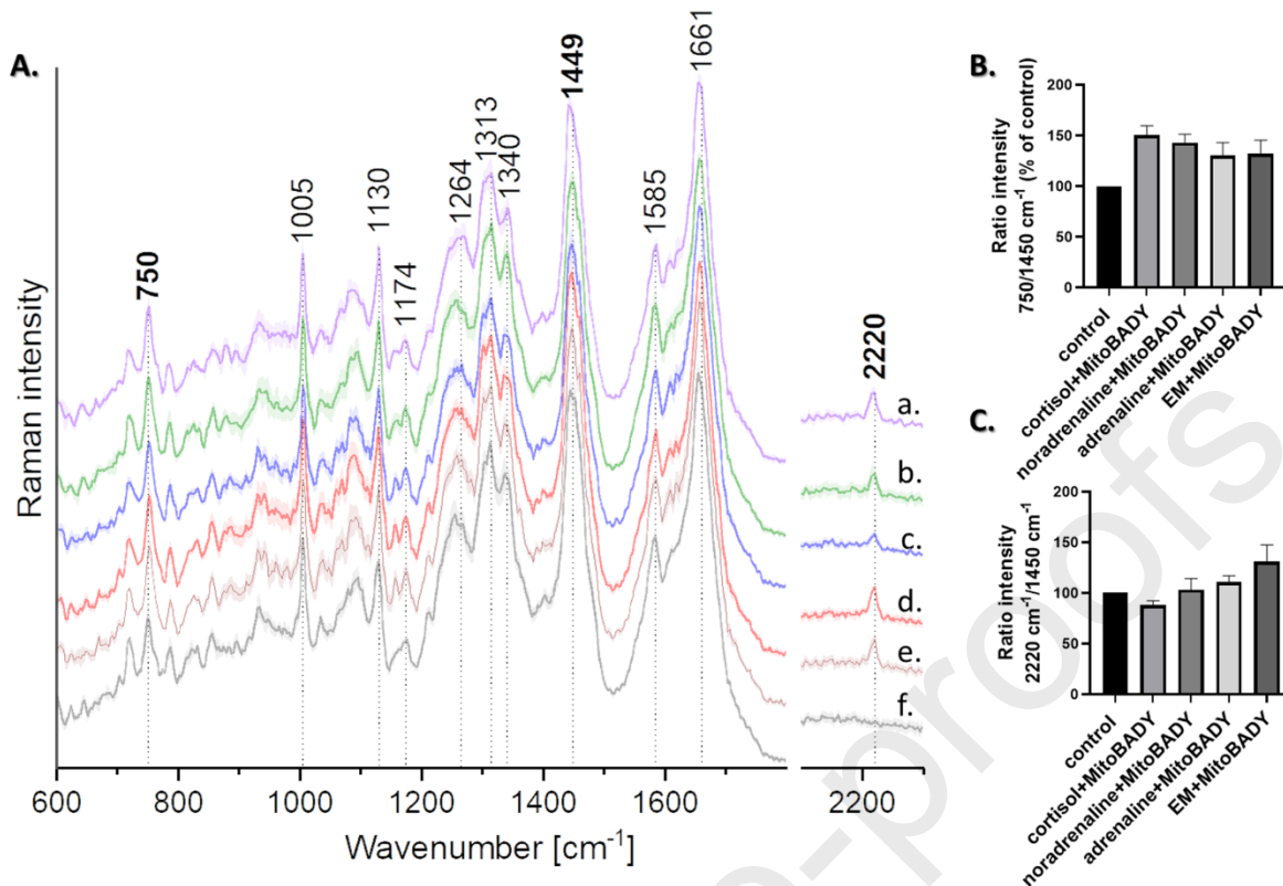
Fig. 7 A. Averaged Raman spectra of cytoplasm region with standards deviation for EM + MitoBADY (a), adrenaline + MitoBADY (b), noradrenaline + MitoBADY (c), cortisol + MitoBADY (d), MitoBADY (e.) and control (f). B. The integral intensity ratio of bands at 750/1450 cm -1 . C. The integral intensity ratio of bands at 2220/1450 cm -1 .
