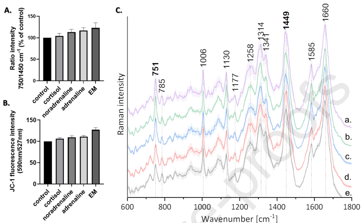
Fig. 6A. The integral intensity ratio of bands at 750/1450 cm -1 . B. The JC-1 fluorescence intensity (ratio of 590 nm/527 nm). C. Averaged Raman spectra of cytoplasm region with standards deviation for EM (a), adrenaline (b), noradrenaline (c) cortisol (d), and control (e).
