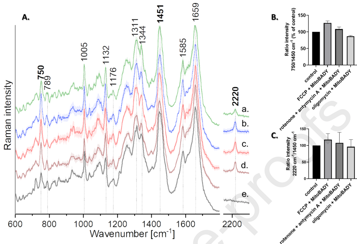
Fig. 5. A. Averaged Raman spectra of cytoplasm region with standards deviation for oligomycin + MitoBADY (a), rotenone and antimycin A + MitoBADY (b), FCCP+ MitoBADY (c), MitoBADY (d) and control (e). B. The integral intensity ratio of bands at 750/1450 \text{cm}^{-1} . C. The integral intensity ratio of bands at 2220/1450 \text{cm}^{-1} .
