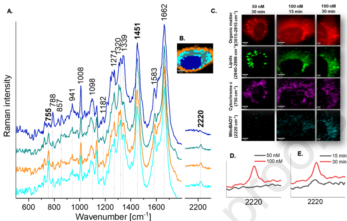
Fig. 3A. KMCA-based average spectra of characteristic classes (a. nucleus, b. cytoplasm region with high content of lipids, c. organic matter, d. cytoplasm region with high content of cytochrome c) and B. cluster maps, the most important of which was the cytoplasm class. Raman imaging of live HAEC cells incubated with MitoBADY. C. Selected experimental conditions: 50 nM, 30min; 100 nM, 15 min; 100 nM, 30 min, obtained by the integration of Raman bands over the selected Raman bands at: 2930 \text{cm}^{-1} (organic matter), 2850 \text{cm}^{-1} (lipids), 750 \text{cm}^{-1} (cytochrome c) and 2220 \text{cm}^{-1} (MitoBADY). Average spectrum showing the differences between the 2220 \text{cm}^{-1} band intensity for D. concentration and E. incubation time.
