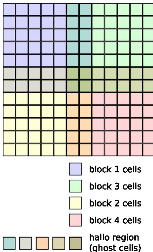
Fig. 2. Block decomposition with 1 cell wide halo region
